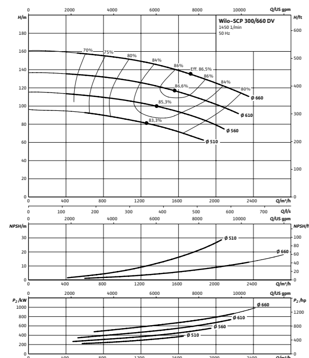
Wilo-SCP 300/660 DV
