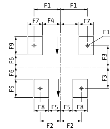
Dimension drawing: Pump base, single-stage version 泵座尺寸图
