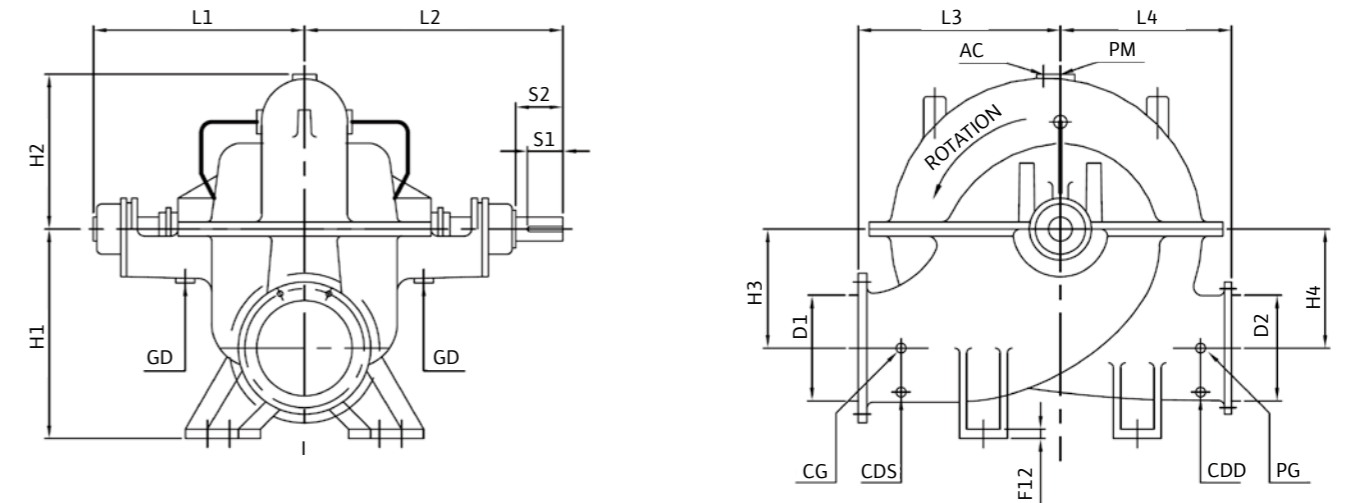
Section drawing: Pump with bare shaft end, single-stage version 泵头外形尺寸图
