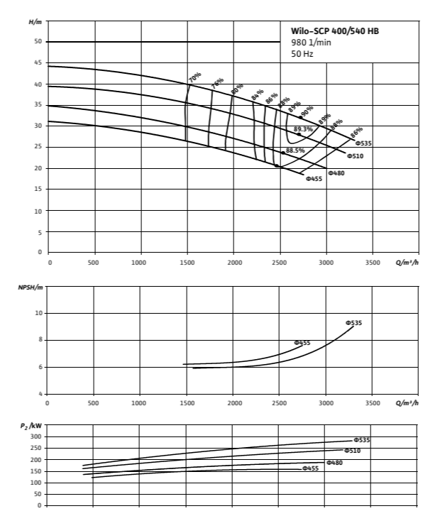
Wilo-SCP 400/540 HB
