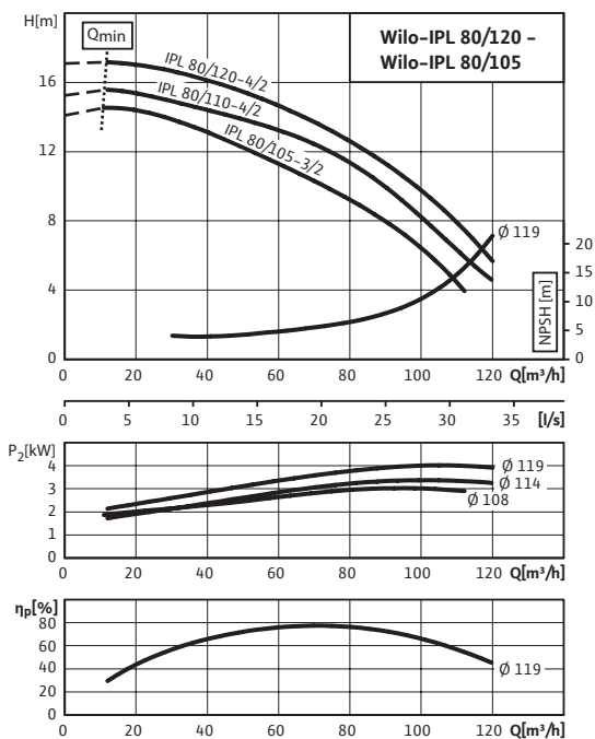
Wilo-IPL 80/105-3/2 - 80/120-4/2
