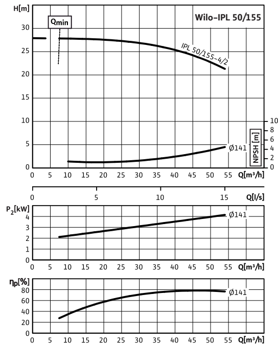
Wilo-IPL 50/155-4/2
