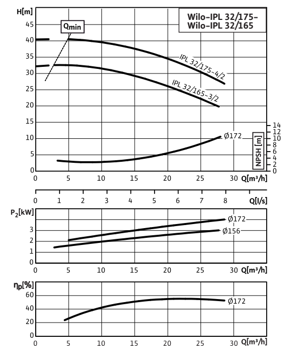
Wilo-IPL 32/165-3/2 - 32/175-4/2
