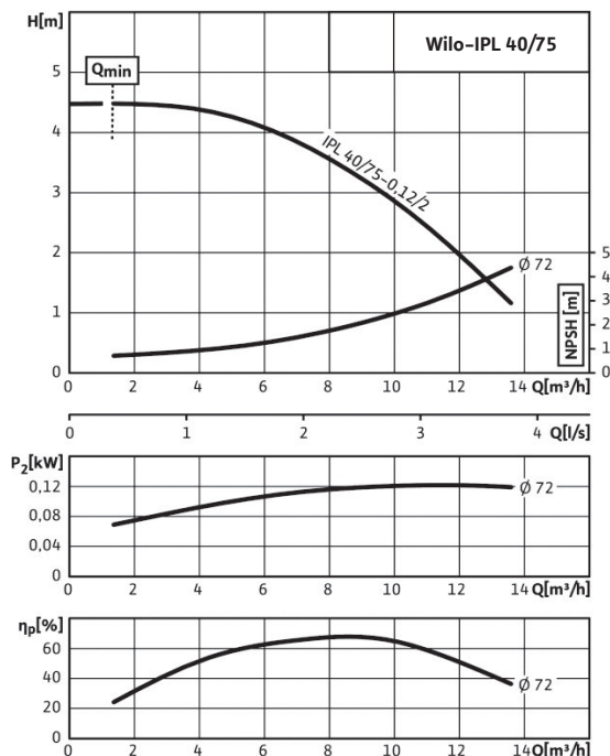
Wilo-IPL 40/75-0.12/2
