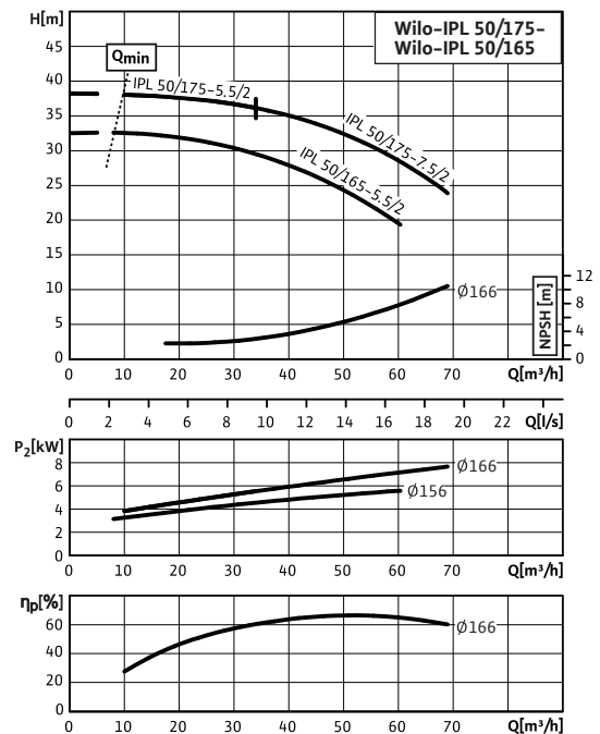
Wilo-IPL 50/165-5.5/2 - 50/175-7.5/2
