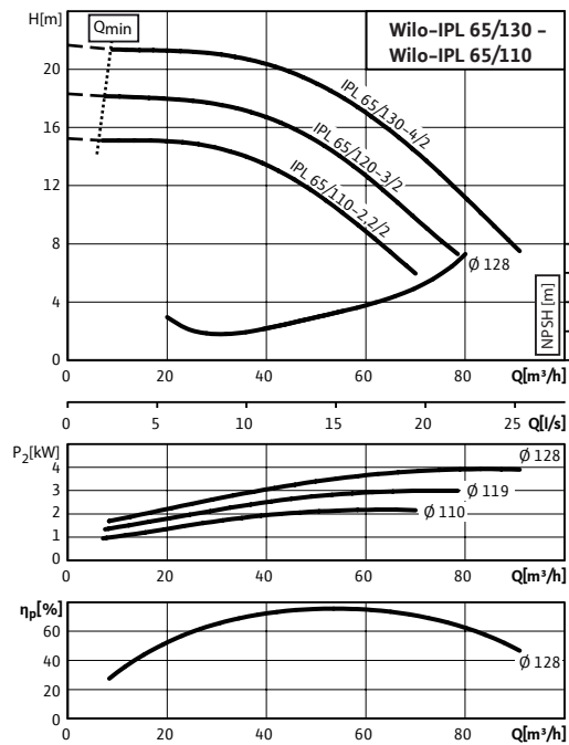
Wilo-IPL 65/110-2.2/2 - 65/130-4/2
