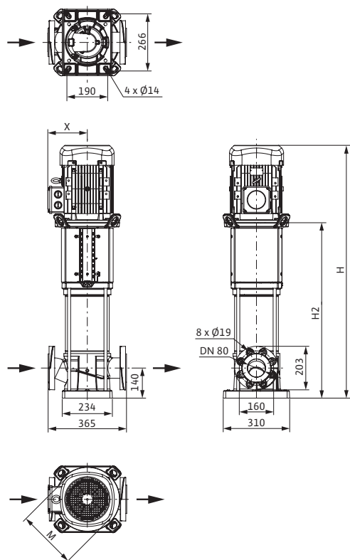
尺寸、重量 Dimensions, weights: Pump housing 1.4308 [AISI304]
