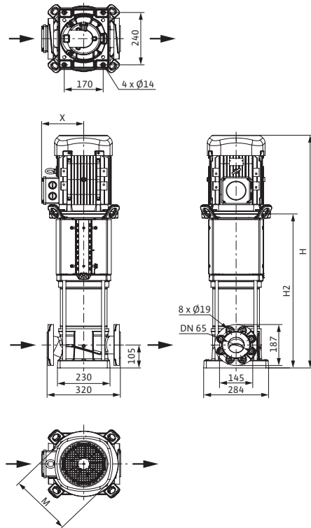
尺寸、重量 Dimensions, weights: Pump housing 1.4308 [AISI304]
