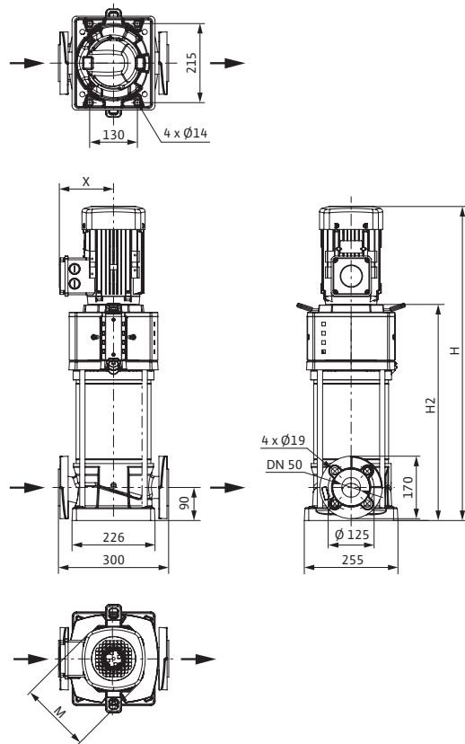
尺寸、重量 Dimensions, weights: Pump housing 1.4308 [AISI304]
