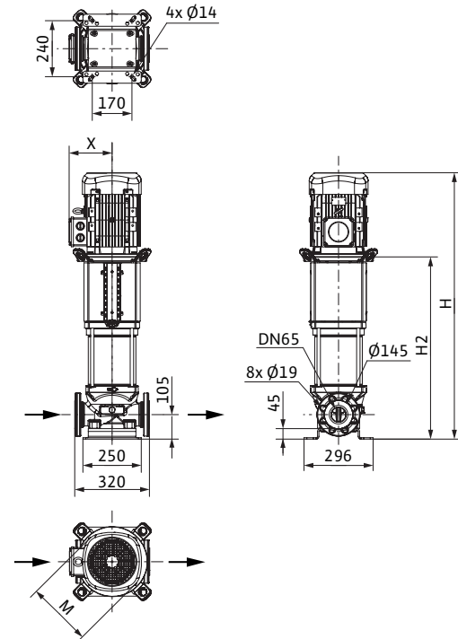
尺寸图 Helix V 36, Pump housing 1.4409 [AISI316L]
