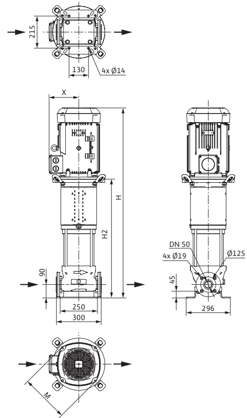
尺寸图 Dimension drawing Helix V 22, PN 25, Pump housing 1.4409 [AISI316L]
