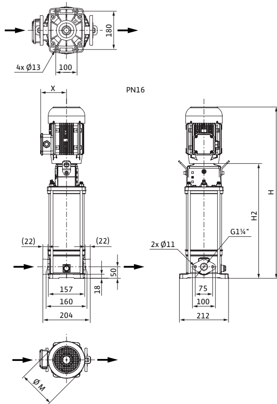
尺寸、重量 Dimensions, weights: Pump housing 1.4301 [AISI304]
