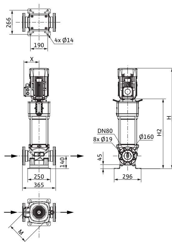
尺寸图 Helix V 52, Pump housing 1.4409 [AISI316L]
