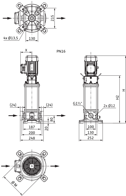
尺寸、重量 Dimensions, weights: Pump housing 1.4301 [AISI304]
