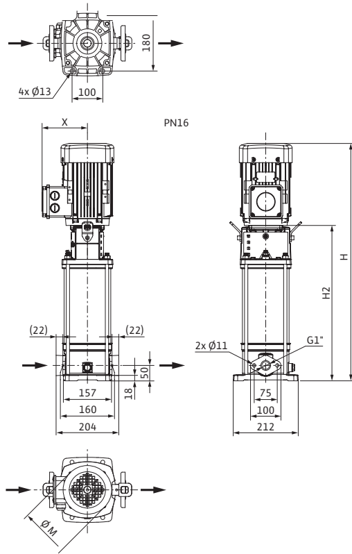
尺寸、重量 Dimensions, weights: Pump housing 1.4301 [AISI304]
